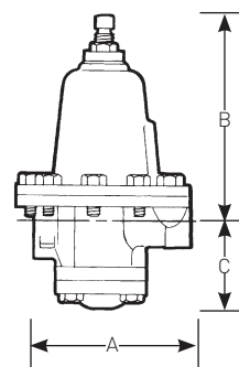
TYPE G-60 Threaded connections
